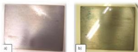
Figure 1: Carbon steel samples exposed to seawater and 0.05% Vapro 844 before (a) and after (b) immersion in ferroxyl indicator.
