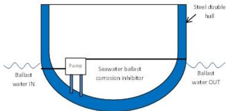
Figure 3. Ballast water tank.
