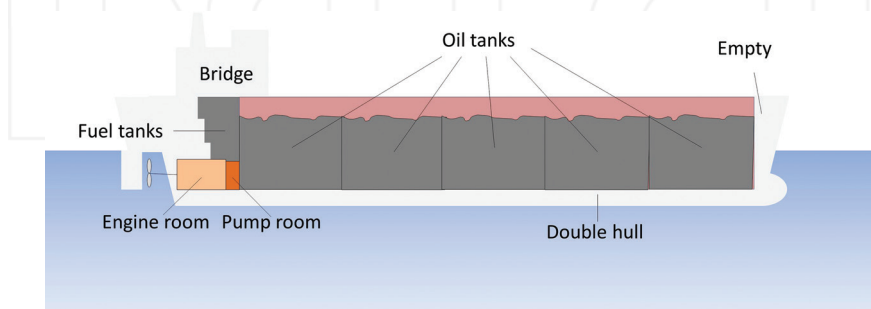
Figure 8. Petroleum transportation tanker showing holds containing ballast water with VCI powder.
