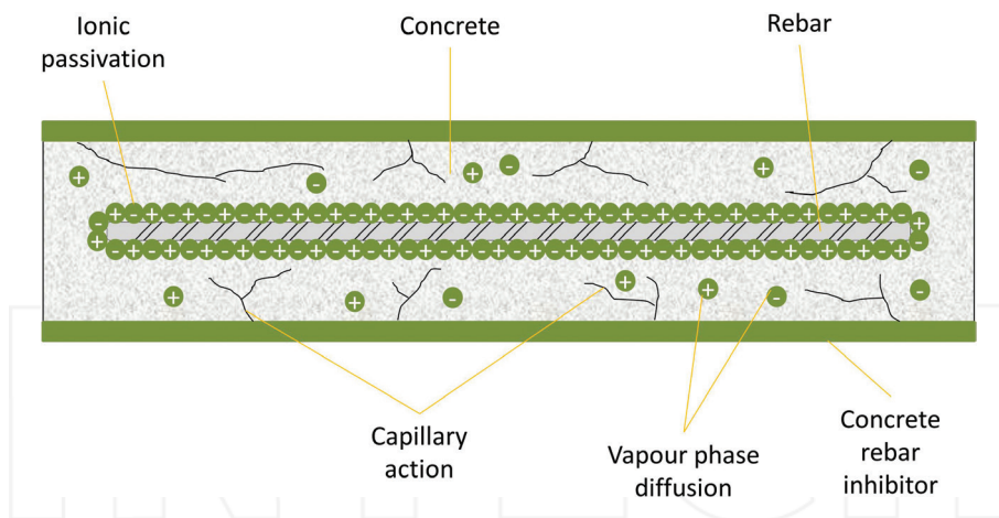
Figure 9. Protection mechanism of the concrete steel rebar.
